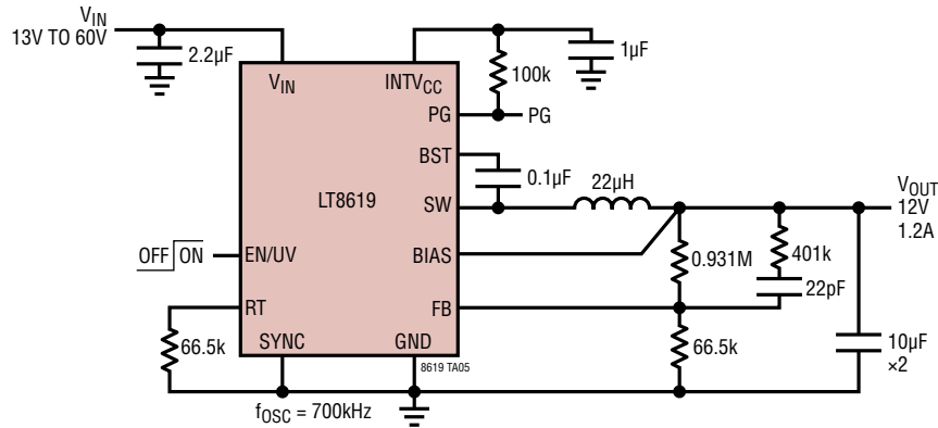
12V 700kHz Step-Down Converter
